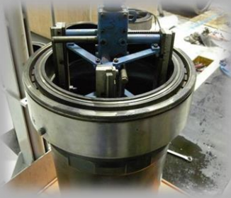
■ CYLINDER LINER ■
